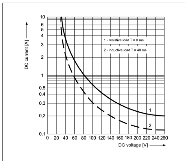
Fig. 22. Maximum switching capacity at direct current
