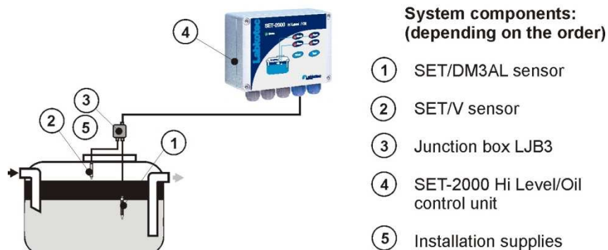
Figure 1. Oil separator alarm system with OilSET-2000 Hi Level/Oil
