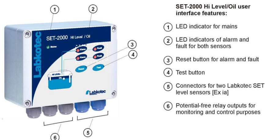
Figure 2. SET-2000 Hi Level/Oil – features
