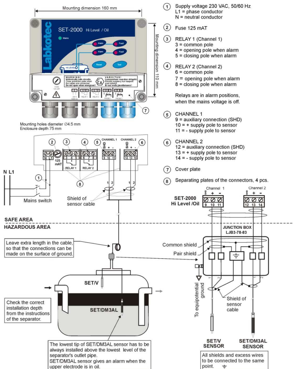
Figure 3. Installation of SET-2000 Hi Level/Oil alarm device.
